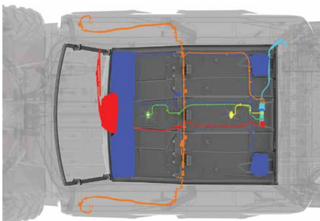
CREW XP 1000 POLARIS PULSE WIRING SHOWN
